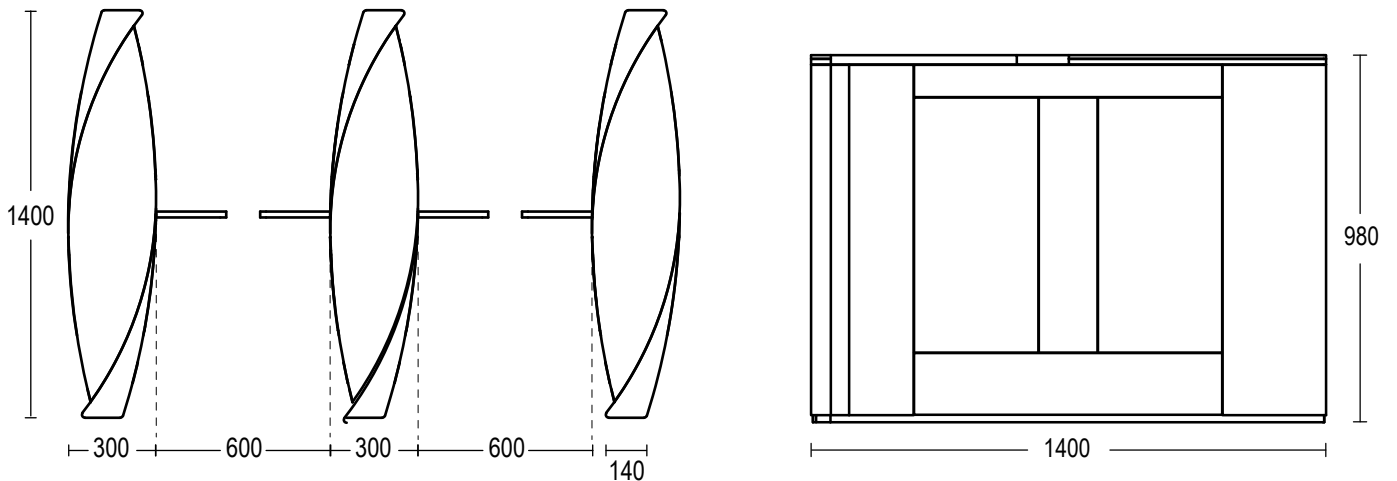
TOP VIEW
